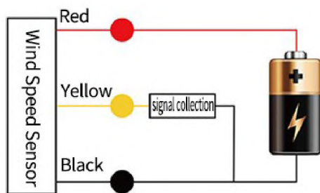
(Voltage signal, 4~20mA)
